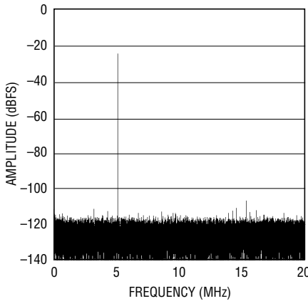
LTC2204: 64K Point FFT, 40Msps, f_{IN} = 5.1\text{MHz} , -25\text{dBFS} , \text{PGA} = 0 , \text{DITH} = 0
